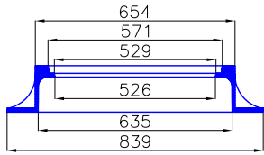
FRAME AND GRATE DETAILS
